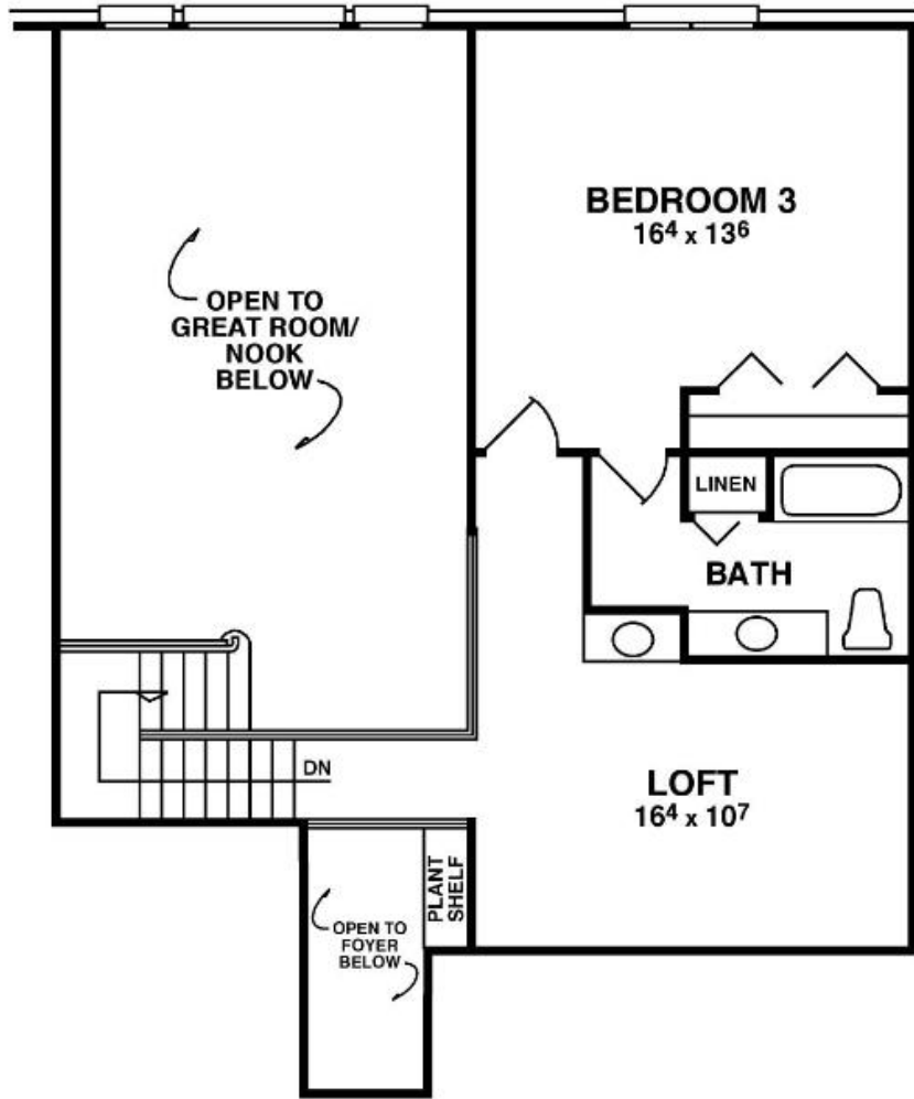
SPLIT SECOND FLOOR PLAN
